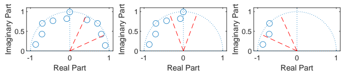
Fig. 6. Local poles for each dominant pole. The red lines represent the frequency range around each dominant pole where f_r = 20Hz .
