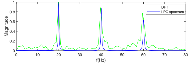
Fig. 2. Spectrum response. The green trace is the result from the discrete Fourier transform and the blue trace is the LPC filter result H(z) , the LPC order is p = 20 .
