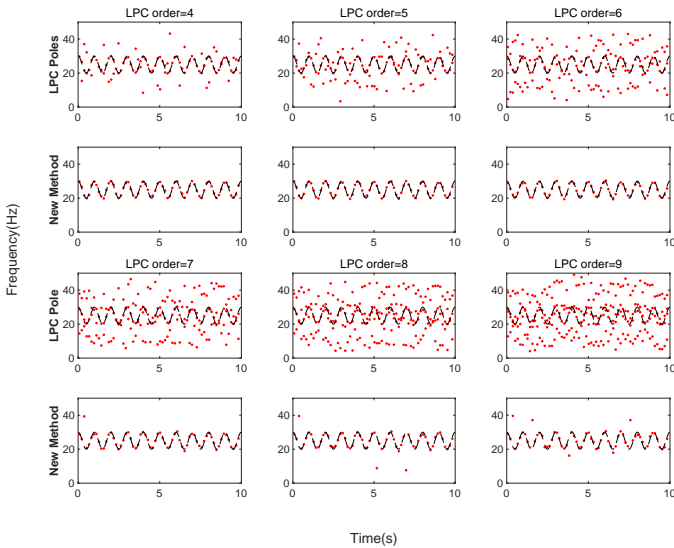
Fig. 11. LPC order analysis. The other parameters are the same as Fig. 10.
