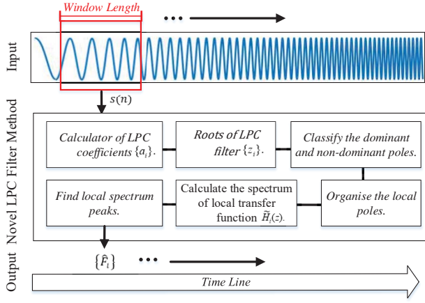
Fig. 8. The overview of the new framework. The first step is to segment the input signal with a fixed window length, then the windowed signal is processed in 6 steps, the output results are the predicted dominant formants at the sample window time.
