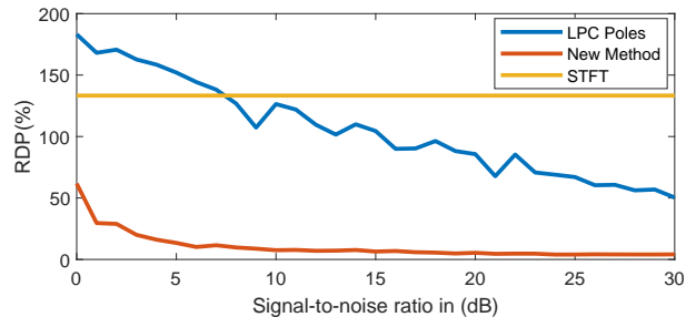
Fig. 14. The RDP for SNR due to AWGN in dB. The number of samples is N = 15 , LPC order is p = 6 , the threshold value c = 0.85 , the frequency range f_r = 15Hz .
