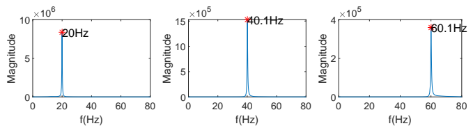
Fig. 7. Local spectrum. The prediction results are \hat{F}_1 = 20Hz , \hat{F}_2 = 40.1Hz and \hat{F}_3 = 60.1Hz .
