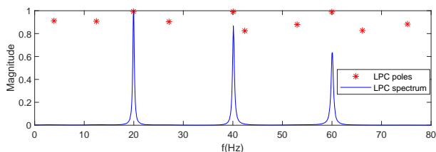
Fig. 4. LPC spectrum and LPC poles.
