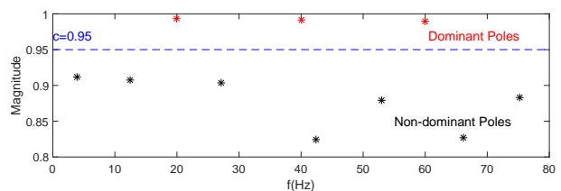
Fig. 5. Dominant and non-dominant poles.
