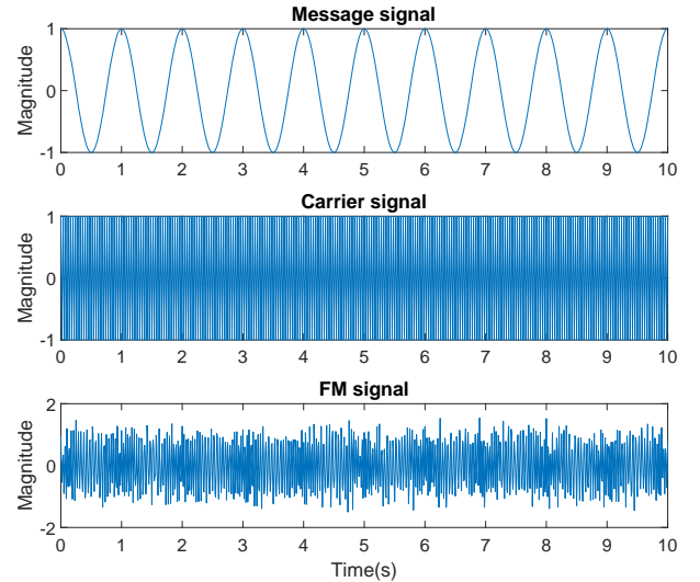
Fig. 9. Single FM signal with SNR=10dB due to AWGN. The sampling frequency F_s = 100Hz , sampling time is 10s, the carrier signal frequency f_c = 25Hz , the message signal frequency f_m = 1Hz , the modulation index \beta = 5 .
