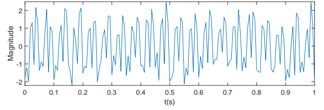
Fig. 1. Input signal. This input signal is composed of F_1 = 20Hz , F_2 = 40Hz , F_3 = 60Hz sine waves where the SNR= 10dB is due to Additive White Gaussian Noise (AWGN), the sampling frequency F_s = 160Hz , the sampling time is 1s.
