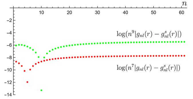
FIG. 1. Log plots showing convergence over n in the mode-sum expression. The red line represents \log(n^7 |g_{nl}(r) - g_{nl}^s(r)|) where we have not included the \mathcal{O}(\epsilon^2) terms in g_{nl}^s(r) (setting m = 1 ). The plot shows that the difference g_{nl}(r) - g_{nl}^s(r) scales like n^{-7} for large n . The green line represents \log(n^9 |g_{nl}(r) - g_{nl}^s(r)|) where we have included \mathcal{O}(\epsilon^2) terms (setting m = 2 ). The plot shows that the difference scales like n^{-9} for large n .
