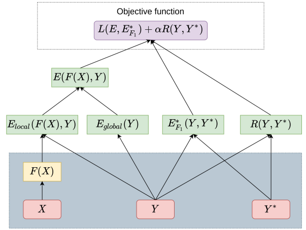
Figure 3: The learning process of our energy-based dialogue state tracker. The grey area denotes a frozen network where the parameters have been pretrained.
