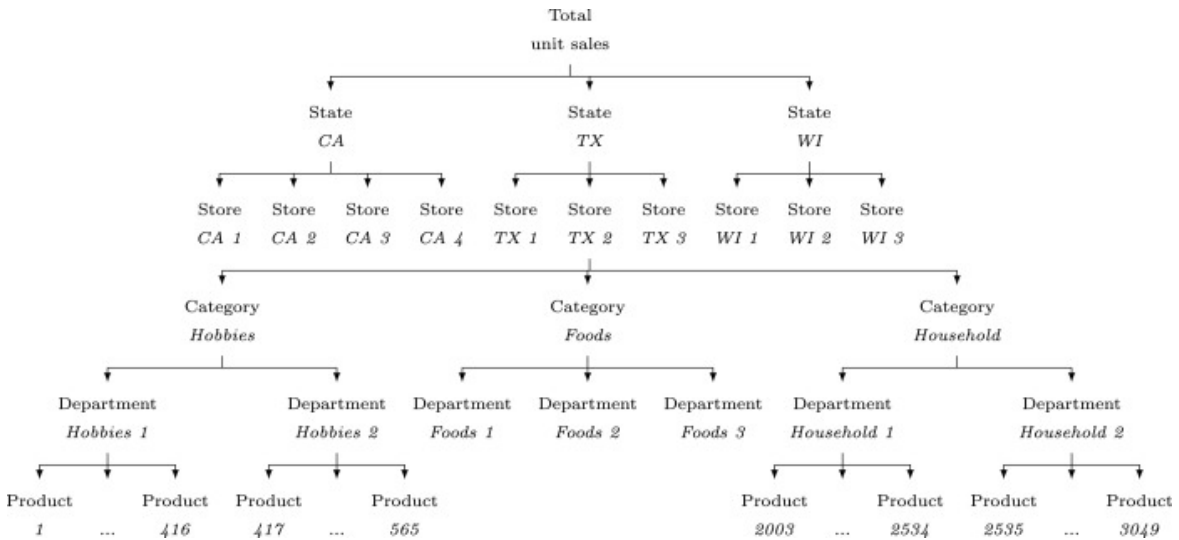
Figure 3.2: M5 products hierarchy. Source: (Makridakis et al., 2022)
