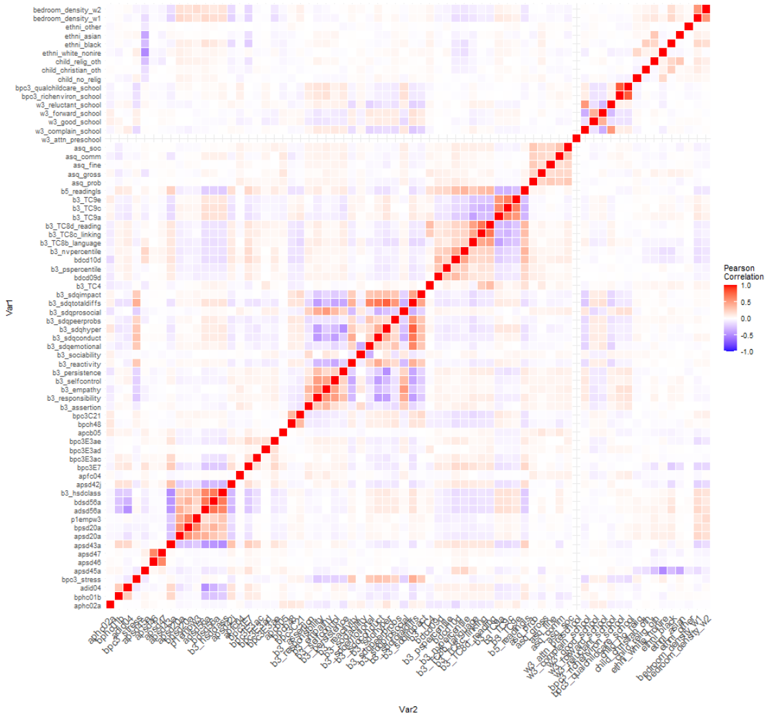
Figure C.1: Pearson correlation heatmap of all variables
