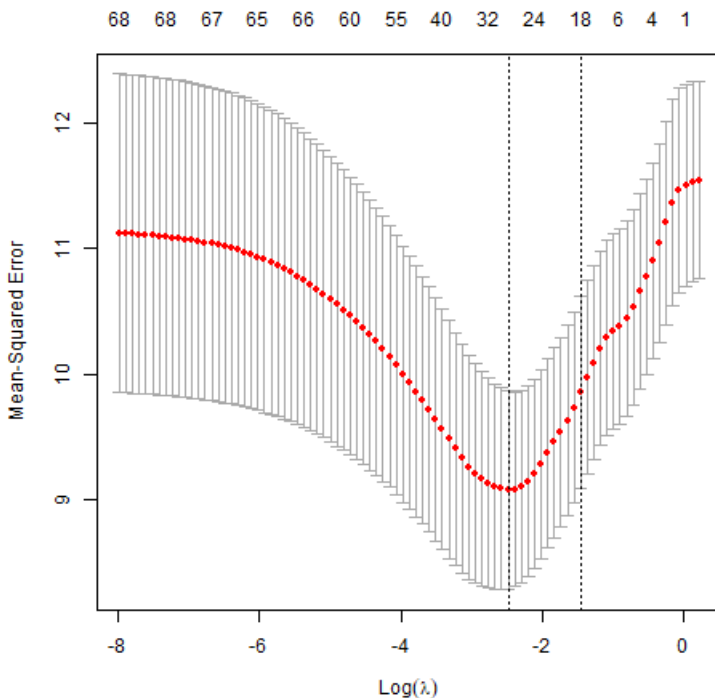
Figure 4.8: Values of the regularisation parameter \lambda . The cross validation curve is shown in red. The upper and lower standard deviations are also shown.
