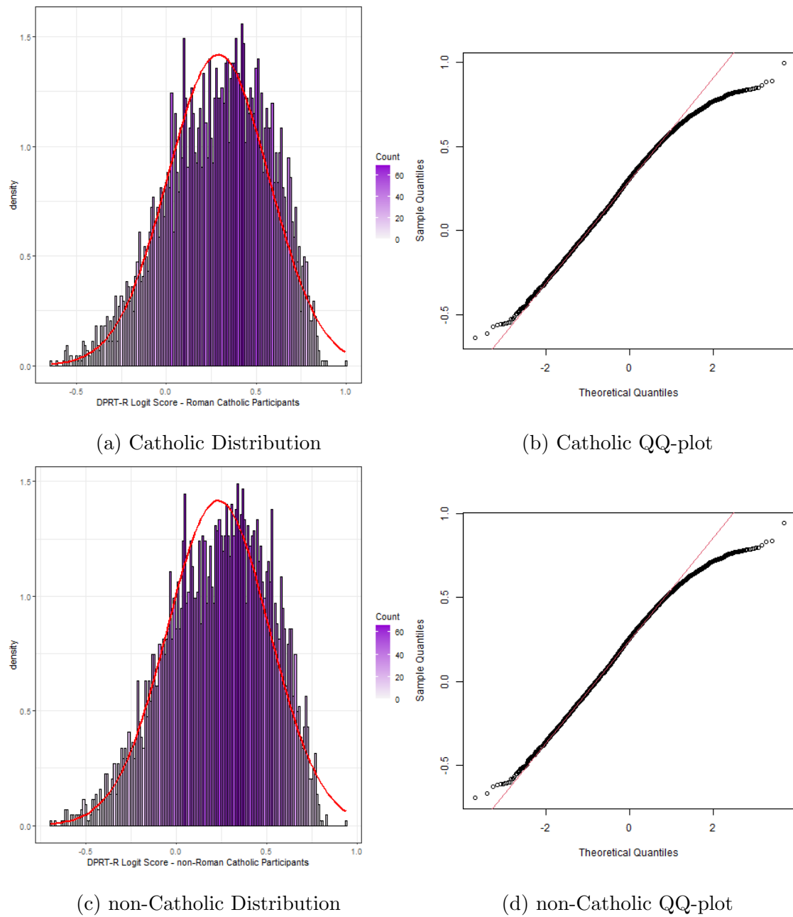
Figure 4.9: Distribution and QQ plots of DPRT-R scores for Catholic and non-Catholic simulated participants
