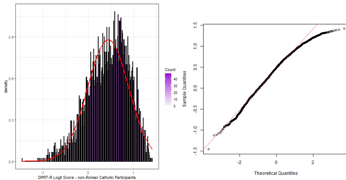
(c) All other ethnicities Distribution (d) All other ethnicities QQ-plot
