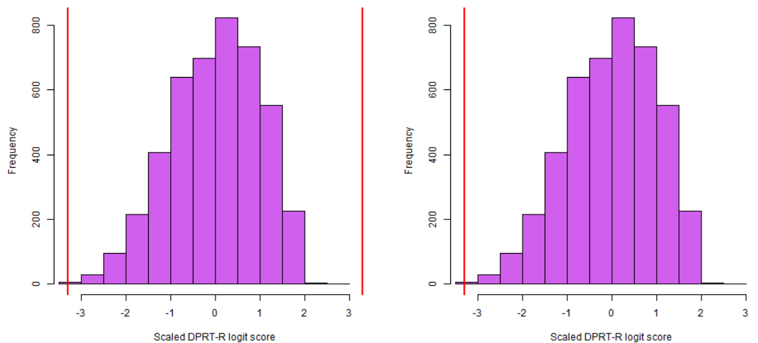
(a) Outliers in Catholic Participants
