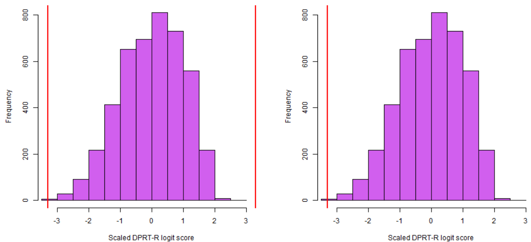
(a) African or other black ethnic background
