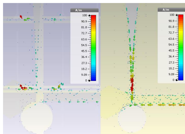
Fig. 4. Antenna Surface Currents for Solar (Left) and Copper (Right)
