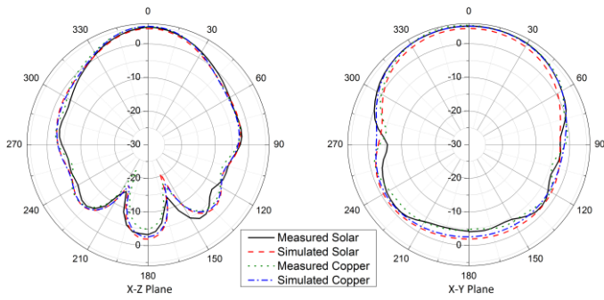
Fig. 7. Radiation pattern at 2.45 GHz
