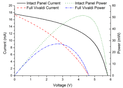
Fig. 9. Solar performance results
