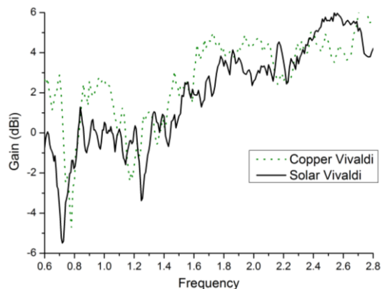
Fig. 3. Measured Boresight Gain
