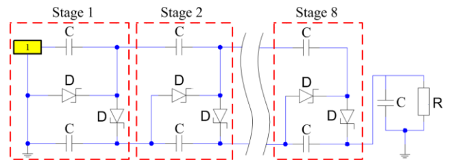
Fig. 10. Villard Cascade Voltage Multiplier Circuit
