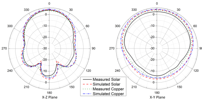
Fig. 6. Radiation pattern at 1.87 GHz
