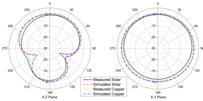
Fig. 5. Radiation pattern at 950 MHz
