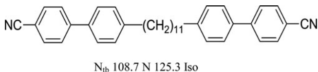
Figure 1. Chemical structure and transition temperature of the material under study: CBC11CB.
