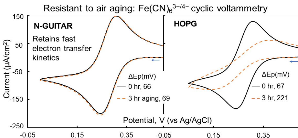
Figure 2. Cyclic voltammograms obtained for the one electron reduction of ferricyanide ions in aerated 0.1 M KCl at 50 mV/s in N-doped amorphous carbon ( left ) and ( right ) in Highly Oriented Pyrolytic Graphite (HOPG) showing a range of \Delta E_p values [31].
