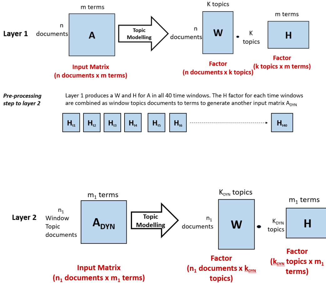
Figure 2.8: Dynamic NMF Topic Model - Layer 1 and 2
