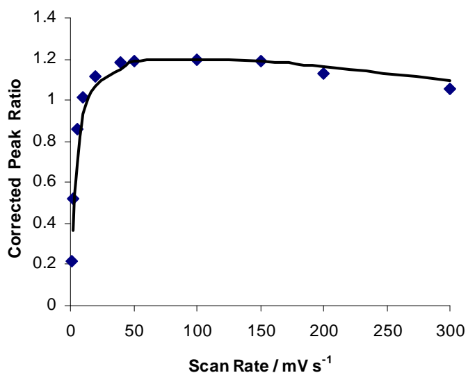
Figure 4.11.a Plot of dimensionless peak current ratio as function of scan rate. Data from Figure 4.7, 4.8, 4.9 and 4.10.
