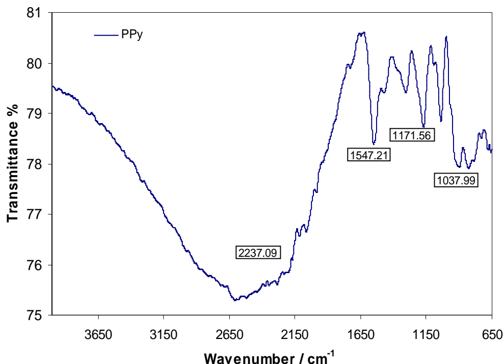
Figure 3.19.C FTIR spectra of PPy film formed in BMIM BF 4 .
