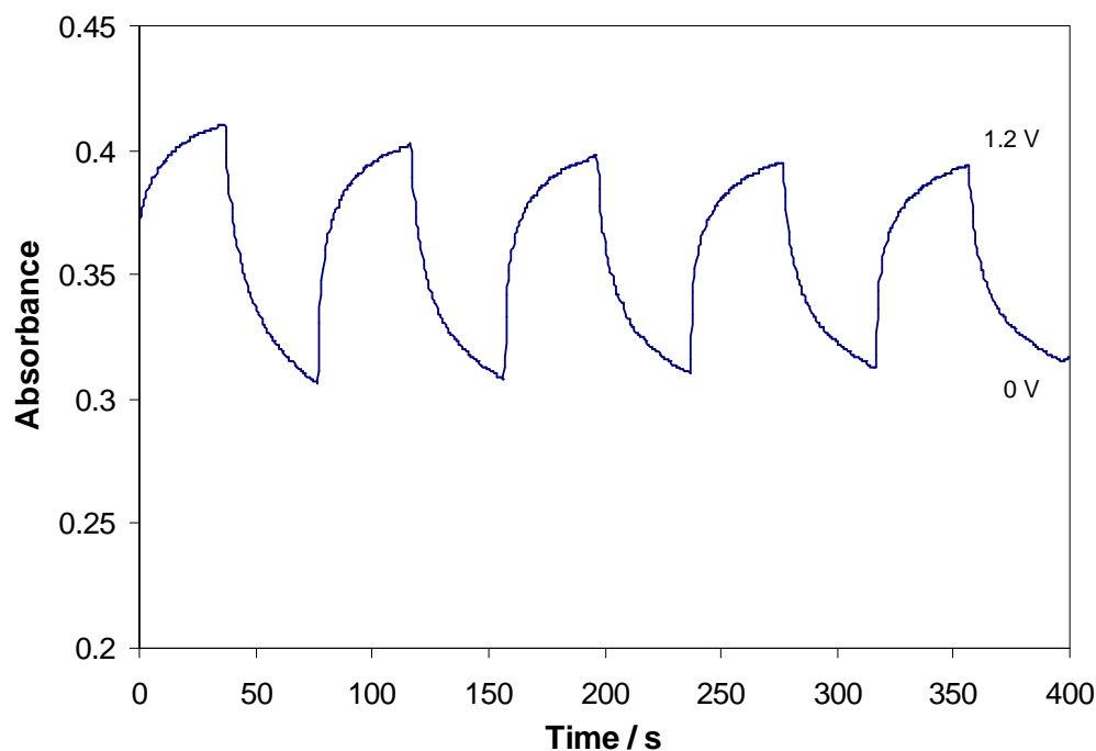
Figure 2.13 Plot of absorbance ( \lambda = 450 \text{ nm} ) versus time of a PTFA film as the potential was switched between 0 V and 1.2 V. The solution contained 2 M \text{HClO}_4 and 50 mM monomer. Switching interval of 40 s.
