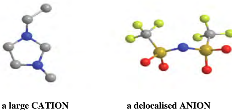
Figure 1.11 Cartoon of two components of an ionic liquid
