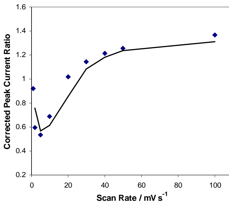
Figure 4.16 Plot of dimensionless peak current ratio as function of scan rate for the cyclic voltammograms performed in phosphate buffer solution pH = 7.0.
