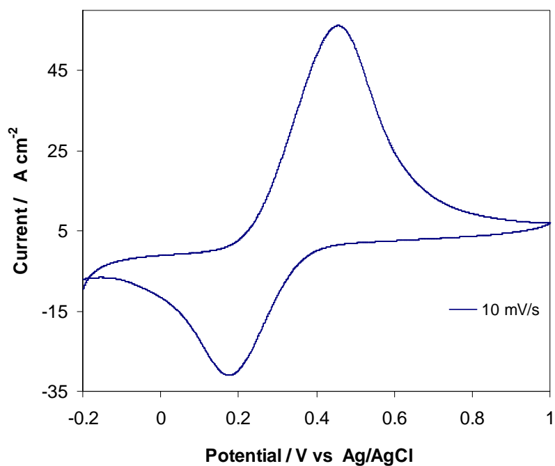
Figure 4.14.d Cyclic voltammogram of Fc/Fc + couple in phosphate buffer (pH = 7.0) solution.
