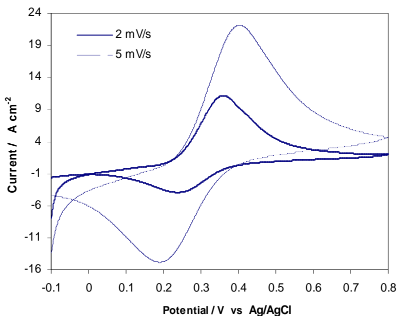
Figure 4.9 Cyclic voltammogram of Fc/ \text{Fc}^+ couple in 0.1 M KCl aqueous solution.
