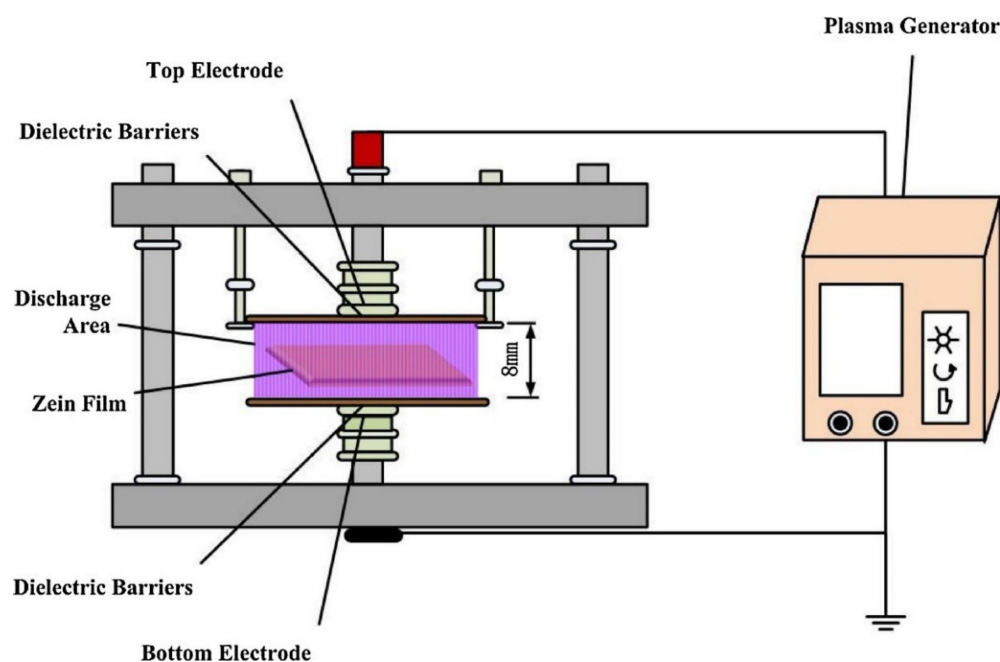
Figure 4. Representation of the experimental setup for treatment of zein films with ACP. Reprinted with permission from ref. [43]. Copyright Elsevier 2022.
