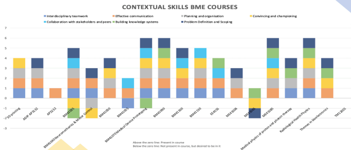
Fig. 6. Contextual skills
