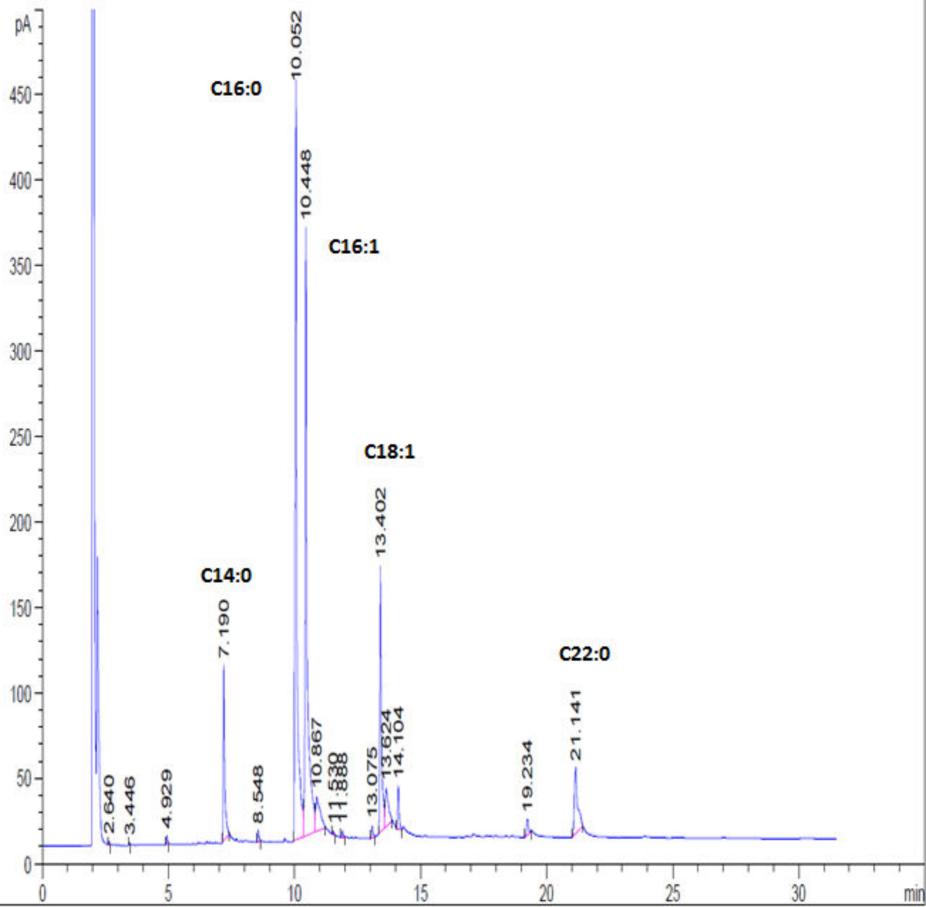
Figure FID1 A, Front Signal (C:\CHEM32\1\DATA\20130501\SIG1000002.D)
