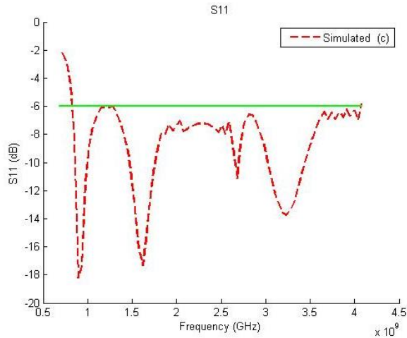
Fig. 2. Simulated S parameter of antenna final antenna element of 1(c)
