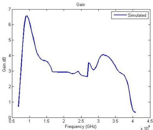
Fig. 7. Simulated Realized Peak gain
