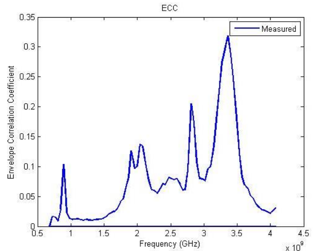
Fig. 9. Measured ECC
