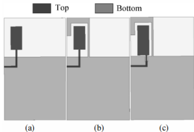
Fig. 1. Three design steps (a) Single antenna element (b) Single element with inverted L structure (c) Optimized antenna element design
