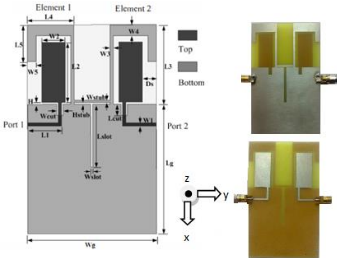
Fig. 3. Geometry of final design and prototype
