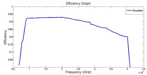
Fig. 8. Simulated Efficiency
