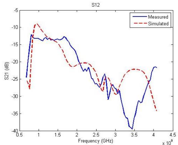
Fig. 5. Simulated and Measured S21
