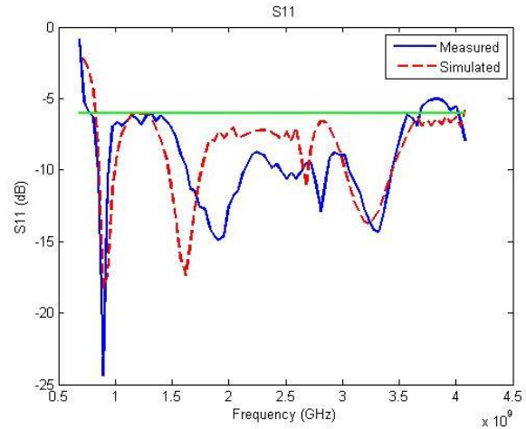
Fig. 4: Simulated and Measured S11
