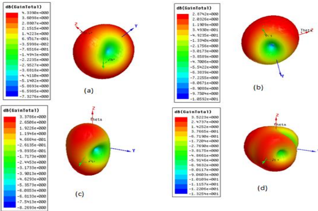
Fig. 6. 3D radiation pattern
