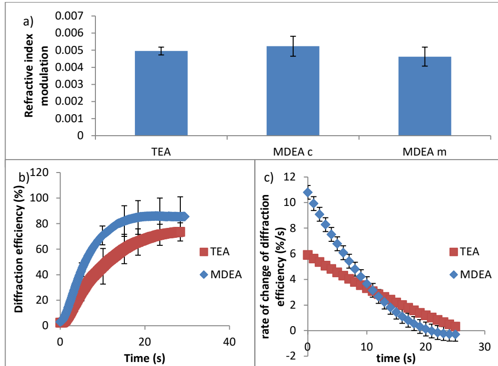
Figure 7. a) Refractive index modulation for each initiator composition. TEA, MDEA (same molar concentration), MDEA (same mass), from left to right (top) b) Growth curves (bottom left) and c) their rate of change of diffraction efficiency for TEA and MDEA with the same molar concentration (bottom right).
