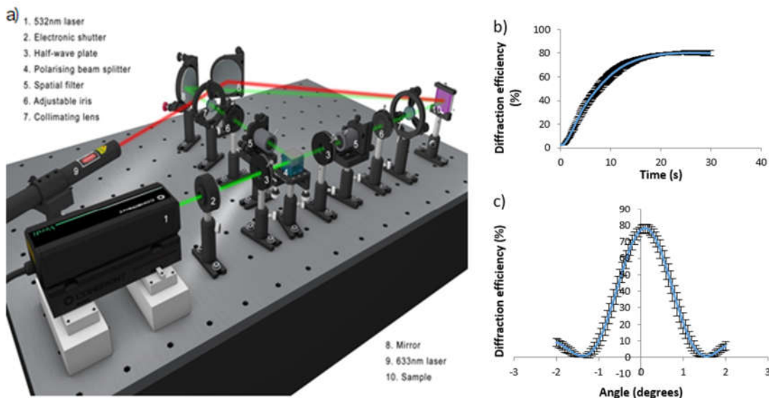
Figure 5. a) Holographic recording (recording beams are shown in green) and real-time monitoring (probe beam are in red) set up; b) Example average growth curve for four samples prepared with 0.592 M acrylamide photopolymer solution; c) Example Bragg curve (bottom).
