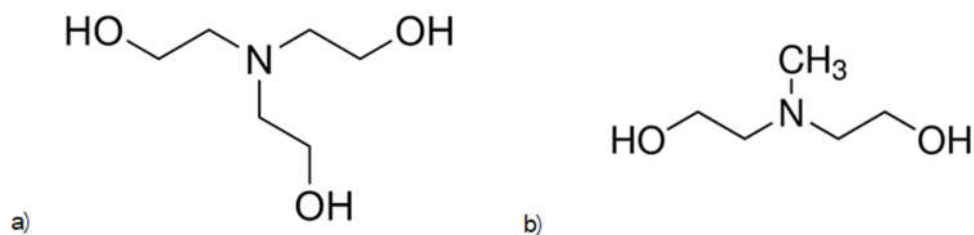
Figure 1. Structure of the studied initiators. a) triethanolamine (TEA) and b) methyldiethanolamine (MDEA).
