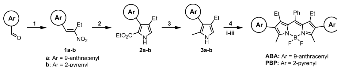
Scheme 1. Synthesis of target compounds. Reagents and conditions: (1) 1-nitropropane (neat), (NH 4 ) 2 CO 3 , reflux, 4–8 h, 59% yield for 1a and 63% yield for 1b ; (2) CNCH 2 CO 2 Et, DBU, THF, room temperature (r.t.), 18 h, 78% yield for 2a and 66% yield for 2b ; (3) LiAlH 4 , THF, reflux, 4 h, 99% yield for 3a and 93% yield for 3b ; (4) (i) PhCHO, TFA, DCM, r.t., 18 h; (ii) DDQ, r.t., 1 h; (iii) BF 3 ·Et 2 O, DIPEA, DCM, r.t., 2 h, 36% yield for ABA , 23% yield for PBP .
