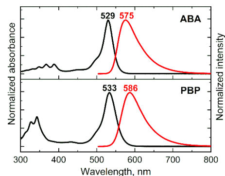
Figure 1. Absorption and emission spectra of ABA and PBP in toluene (λ exc = 490 nm).
