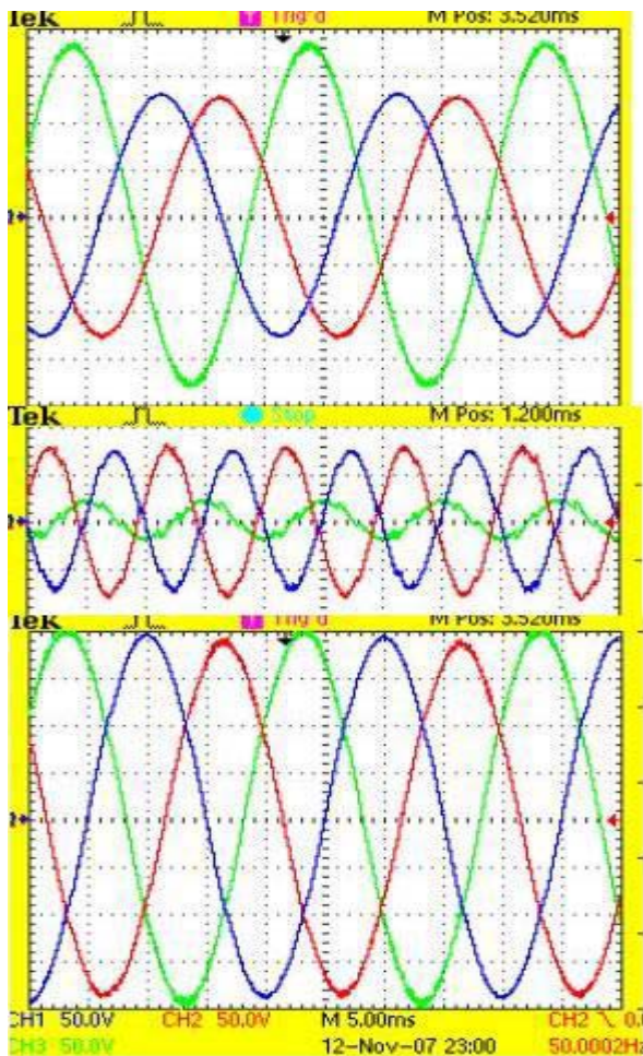
Fig. 10. Source, injected and load voltage during a unbalanced sag (experiment)
