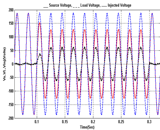
Fig. 6. A phase source, load and injected voltage (simulation)
