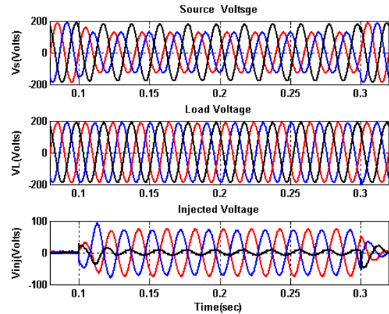
Fig. 7. Source, load and injected voltage during a unbalanced sag (simulation)
