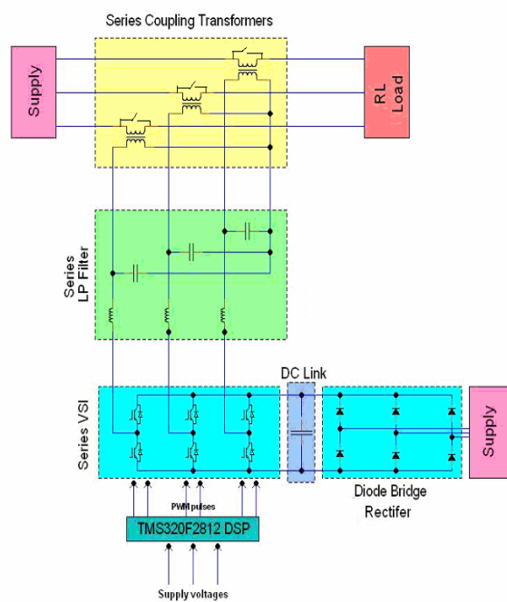
Fig. 1. Power circuit of DVR
