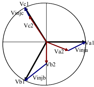
Fig.2. Voltage Phasor
