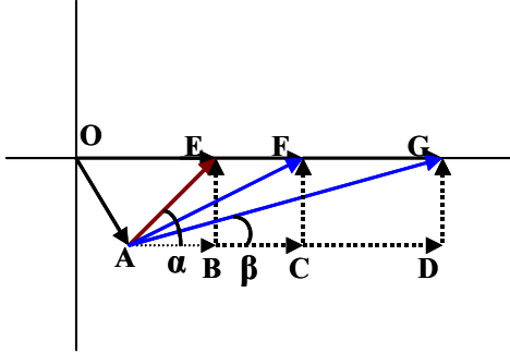
Fig. 3. Injected voltage vector calculation
