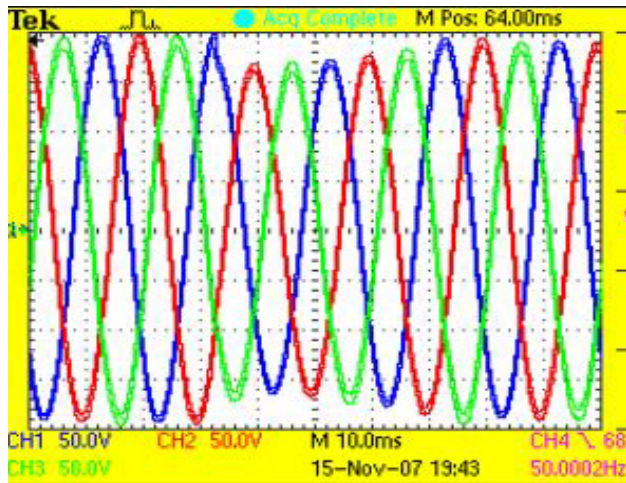
Fig. 9. Load voltage transients during voltage sag (experiment)
