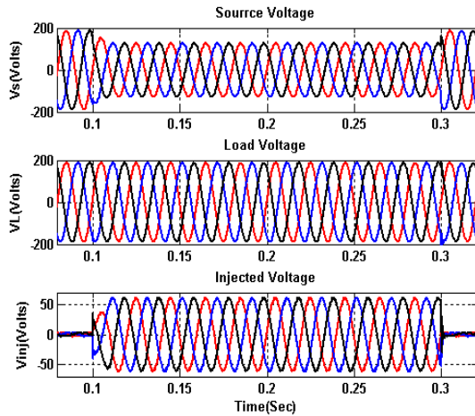
Fig. 5. Source, load and injected voltage during a balanced sag (simulation)
