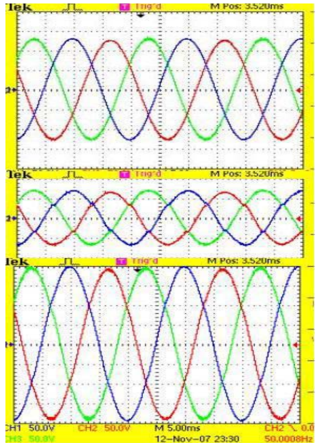
Fig. 8. Source, injected and load voltage during a balanced sag (experiment)
