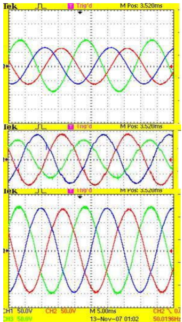
Fig. 11. Source, injected and load voltage during a unbalanced sag with limited injection (experiment)
