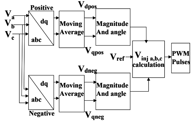
Fig. 4. Control Block of DVR
