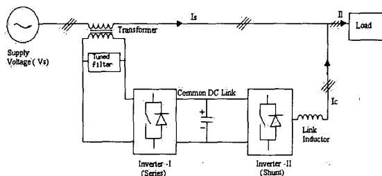
Fig.1 Schematic diagram of UPQC-Q
