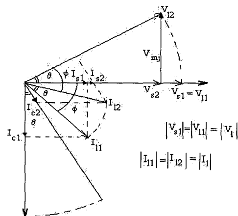
Fig.2 Phasor diagram
