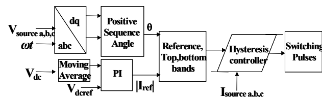
Fig. 2. Control Block of ShAF
