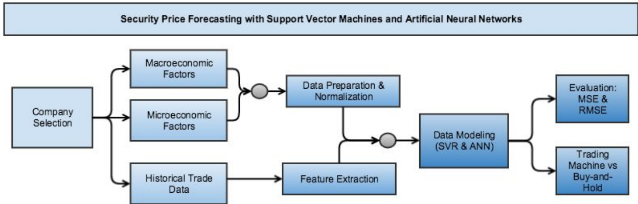
Figure 3.1 provides an overview of the design architecture for evaluating the efficacy of technical indicators used in Support Vector Machines and Artificial Neural Networks. In addition to addressing the company selection process, the macro- and microeconomic indicators and the process for deriving technical features, data modeling and trading machine algorithms are addressed in detail.
