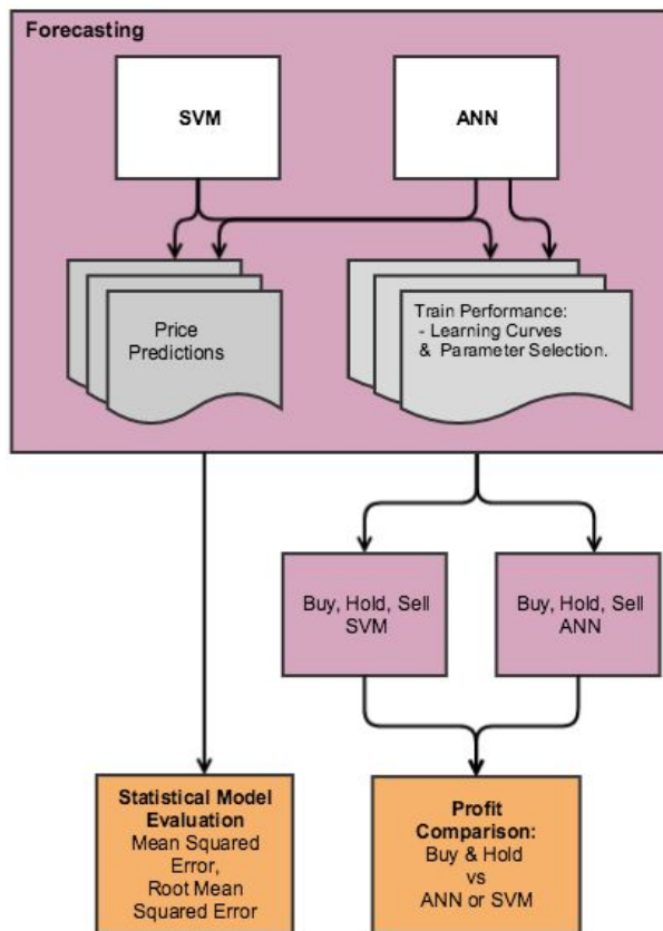
Figure 3.3 illustrates the model pipeline for training, testing and evaluating model performance.
