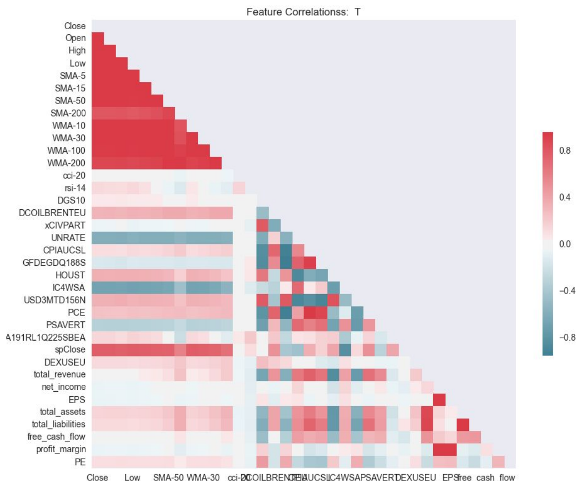
Figure 4.2, showing AT&T, is a correlation-based heat map for all features used in the experiment. As one might expect, there is a very strong correlation between the historical moving prices and the actual Close price, since Close is used for calculating the moving average itself. There is only a moderate to negligible correlation between other technical features such as the CCI and RSI. This is common across all securities in the study.
