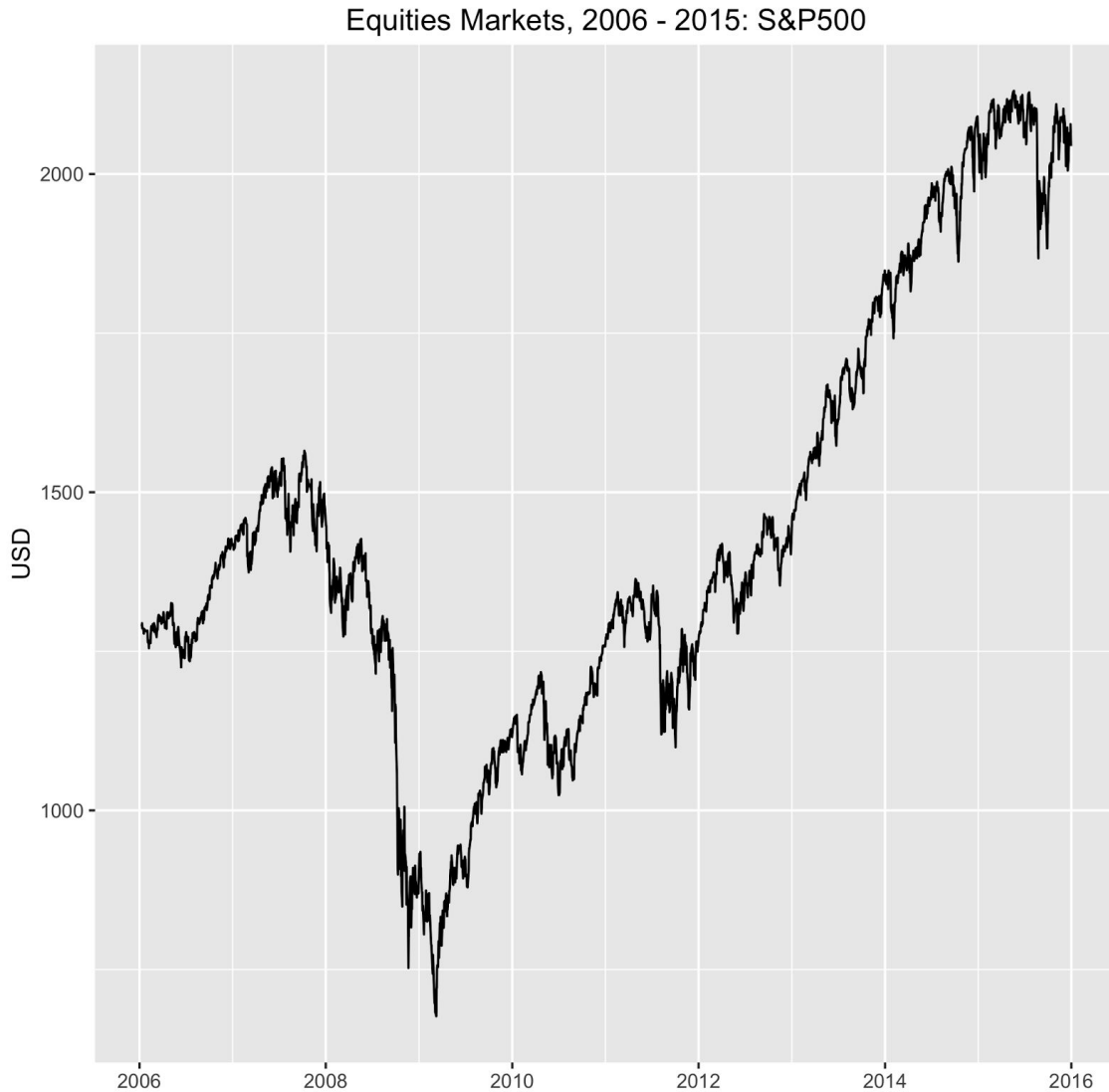
Figure 3.2 provides a historical view of the S&P500, a frequently used index for conceptualizing the growth or diminishment of the US economy as represented by the increase or decrease in the valuation of its largest corporate entities. Data span from 2006 to 2016 and include the sharp decline in the S&P500 which began at the end of 2007 and accelerated its decline into 2008, finally reaching its lowest point in the first quarter of 2009.
