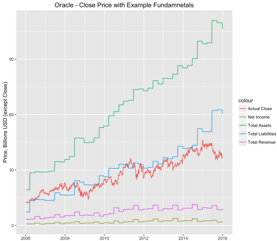
Figure 4.3 shows a the price of Oracle over time in relation to the changing microeconomic fundamentals. As one would expect, the security price (red) increases as net income increases, showing that indeed a security is rationally justified by the performance of the business.
