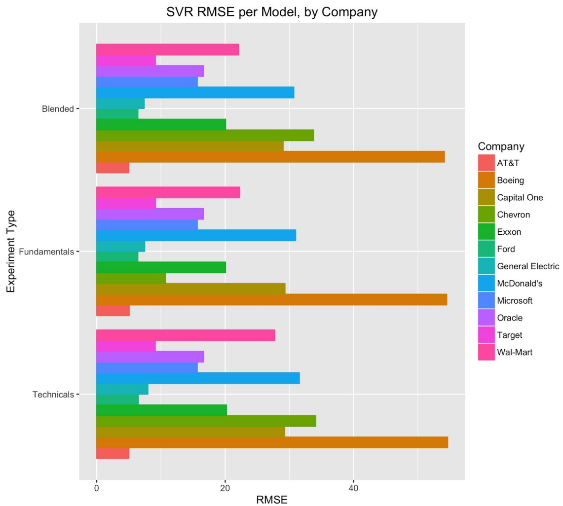
Figure 4.8 illustrates the RMSE for each of the three experimental SVR models for each company included in the study.
