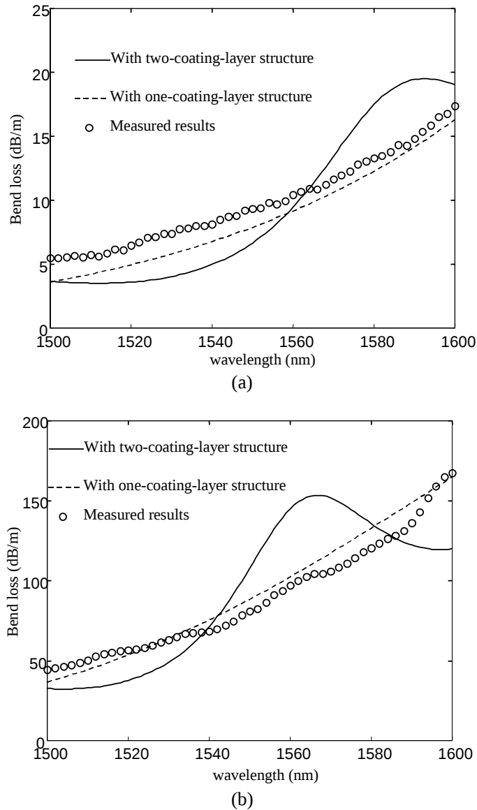
Fig. 5. Calculated (with one-coating layer and with two-coating layers, respectively) and measured bend losses in wavelength range from 1500 nm to 1600 nm for a) for R=10 mm and b) R=9 mm.
