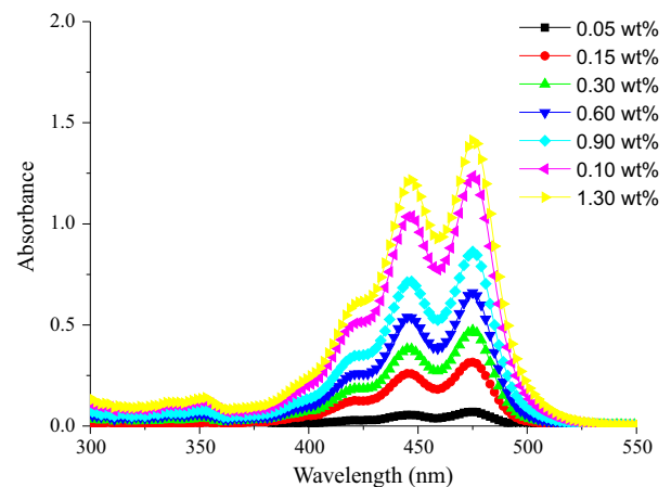
Fig. 2. Absorbance spectra for lumogen yellow day LDS layers of different concentrations.
