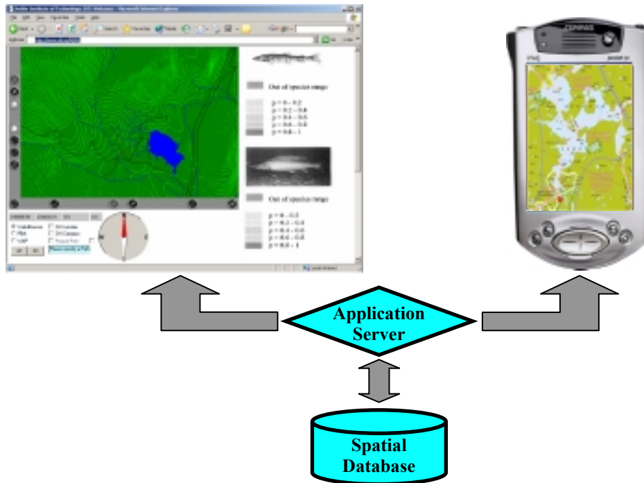
Figure 1: Three-tier Architecture
