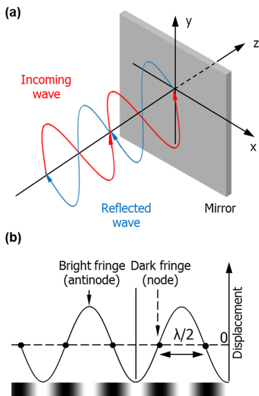
Figure 3. Principle of a (a) standing wave and (b) its corresponding interference pattern.
