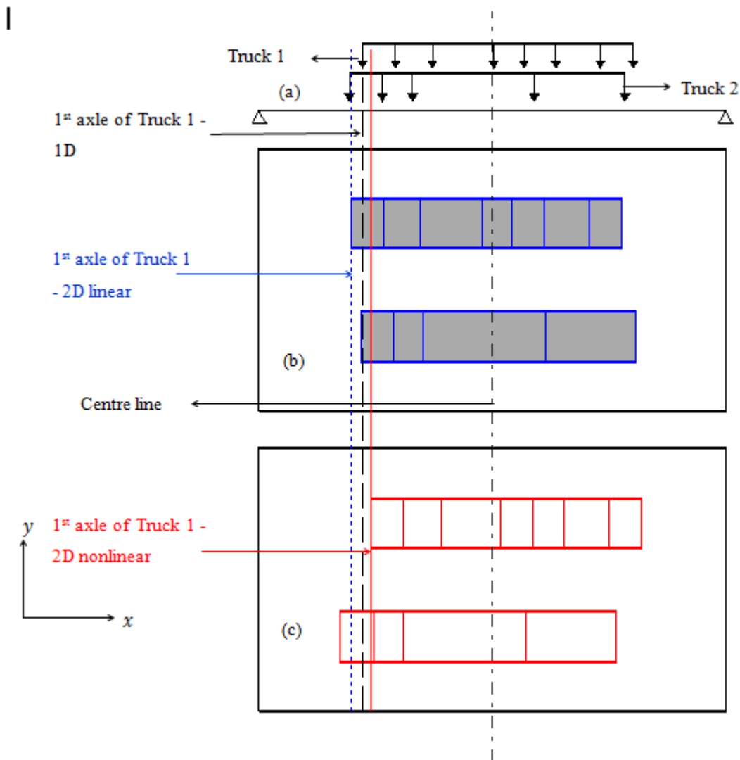
Figure 4 Axle position at critical case (minimum load ratio): (a) 1D linear analysis; (b) 2D linear analysis; (c) 2D nonlinear analysis – 20 m bridge, Czech Republic
