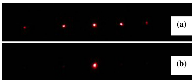
Figure 7 Diffraction patterns for 300 lines/mm at V=0\text{V}/\mu\text{m} (a) and at V=4\text{V}/\mu\text{m} (b).
