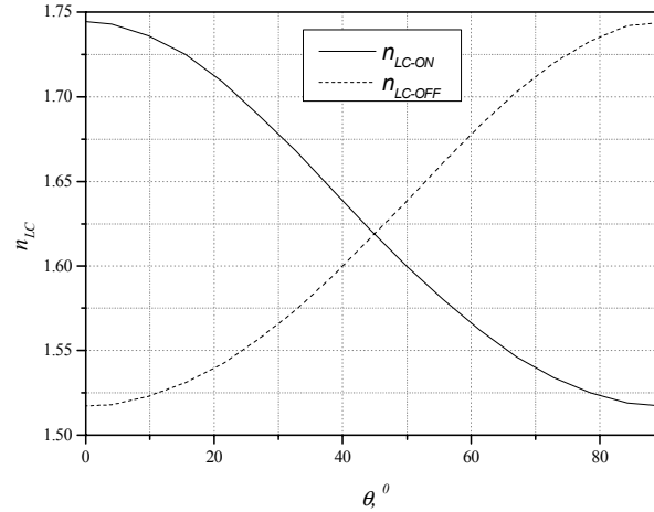
Figure 4. Calculated dependencies of refracting indices on the angle of incidence for OFF and ON modes.
