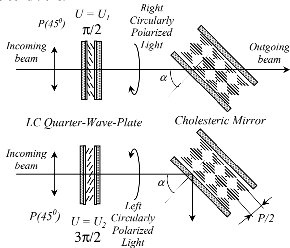
Figure 2. Cholesteric mirror switch schematic diagram.
