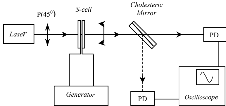
Figure 6. Cholesteric mirror experimental set-up: P – polarizer, PD – photo-diode.
