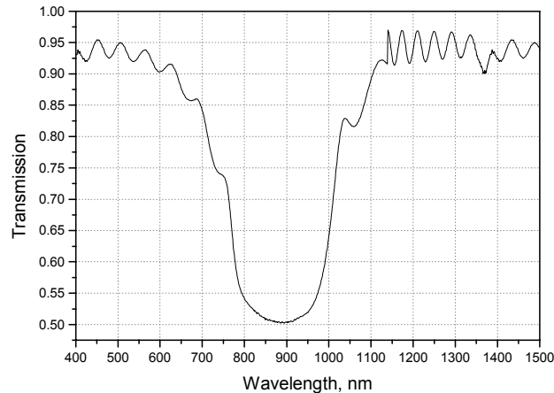
Figure 7. Transmission spectra of the cholesteric mirror sample designed to function at the radiation wavelength of \lambda = 633 \text{ nm} by the angle of 45^\circ .
