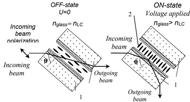
Figure 3. Total reflection switch structure: 1- glass prisms; 2- liquid crystal layer.
