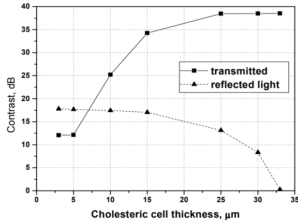
Figure 9. Switching contrast versus the cholesteric cell thickness.
