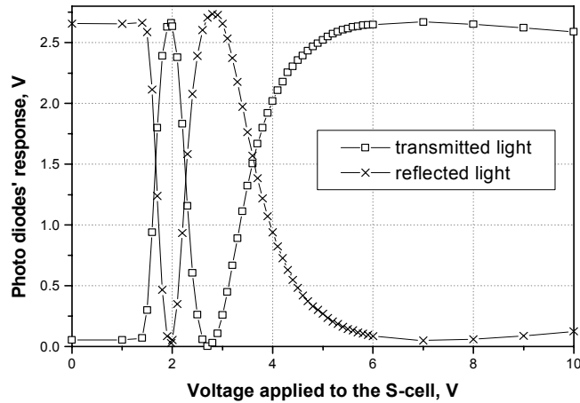
Figure 10. Electro-optic responses for the switch based on the 8 \mu\text{m} cholesteric mirror sample.
