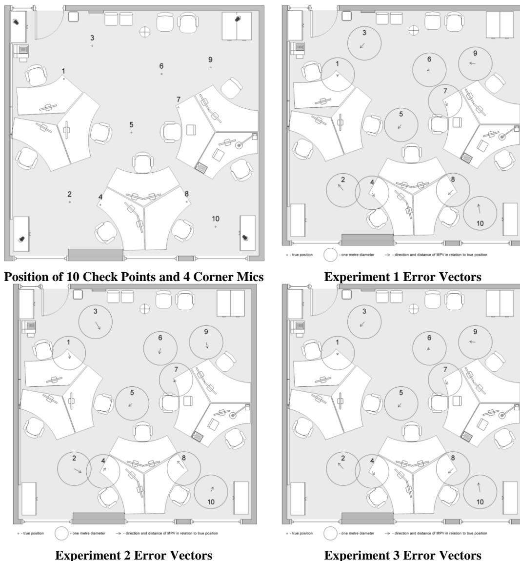
Figure 3. The position of 10 test locations or check points (centerpoint of 1 m diameter circles) and error vector direction and distance from true position to MPV for Experiments 1, 2, and 3.
