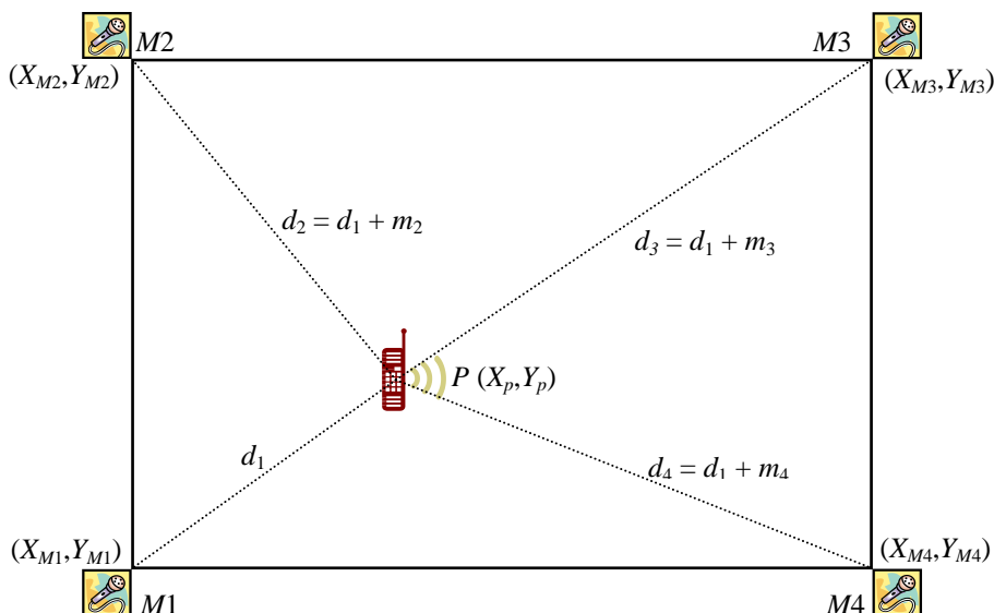
Figure 1. Time Difference of Arrival Trilateration. Control points M1, M2, M3 and M4 are known microphone positions. Point P is the unknown mobile phone’s position, coordinates of which we are trying to find. Lines d_1, d_2, d_3 and d_4 are unknown distances between the phone and each microphone. However, what are known are the differences between the three measurements: m_2, m_3 and m_4 .
