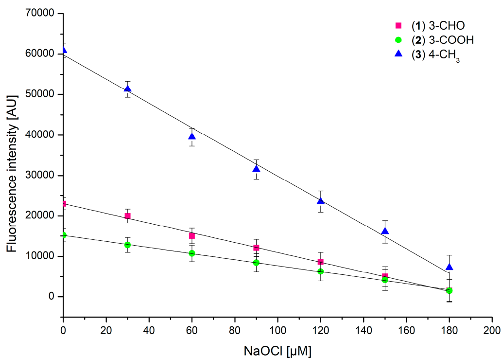
Figure 2. Changes in fluorescence intensity of 150 μM of 1–3 induced by an increase in NaOCl concentration, at pH 5, \lambda_{Ex} 289 nm ( \lambda_{Em} 464 nm, 460 nm, and 450 nm, respectively), and a temperature of 25 °C.
