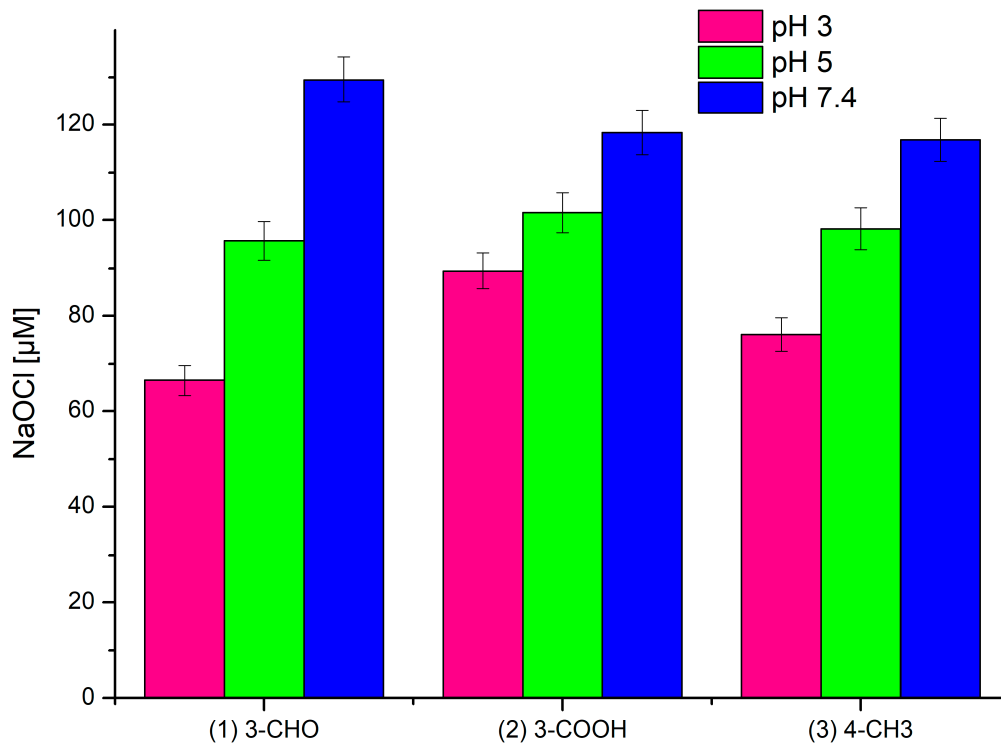
Figure 3. NaOCl concentration causing a 50% decrease in the fluorescence intensity of 150 μM of probes 1–3 at various pH levels, \lambda_{Ex} 289 nm ( \lambda_{Em} 464 nm, 460 nm, and 450 nm, respectively), and a temperature of 25 °C.
