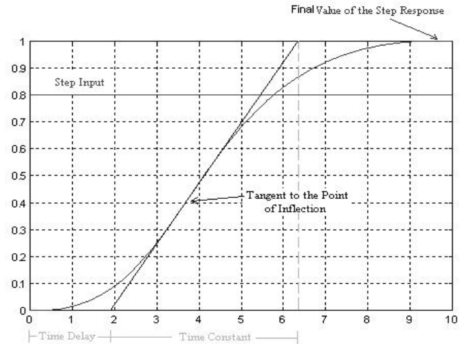
Figure 4. Tangent and point method [20] for developing a process model. K_m = model gain = ratio of the steady state change in process output to steady state change in process input, T_m = model time constant and \tau_m = model time delay. 54 controller tuning rules have been identified based on the model parameters determined from this modelling method. 21 of the 47 other modelling methods for determining such a process model, prior to specifying tuning rules, are based on data gathered from the open loop process step or impulse response [17].
