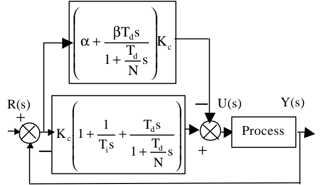
Figure 3. Non-interacting controller, based on the two degree of freedom structure, in a unity feedback block diagram representation. Also labelled the m-PID or ISA-PID controller [17], 44 tuning rules have been identified for this controller structure.
