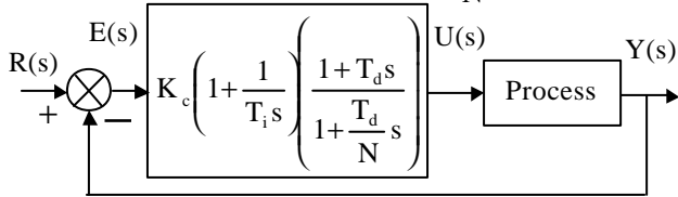
Figure 2. Classical PID controller in a unity feedback block diagram representation. Also labelled the cascade, interacting, series, interactive, rate-before-reset or analog controller [17], 101 tuning rules have been identified for this controller structure.
