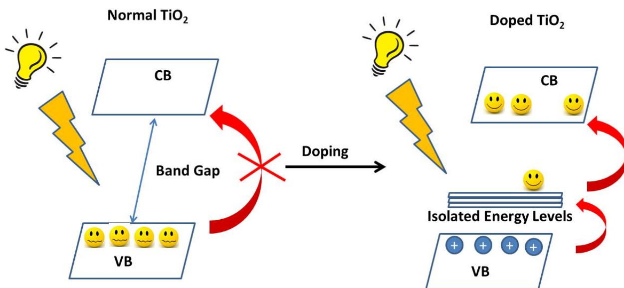
Figure 22. Schematic mechanism of band gap narrowing in anion doped TiO 2 .
