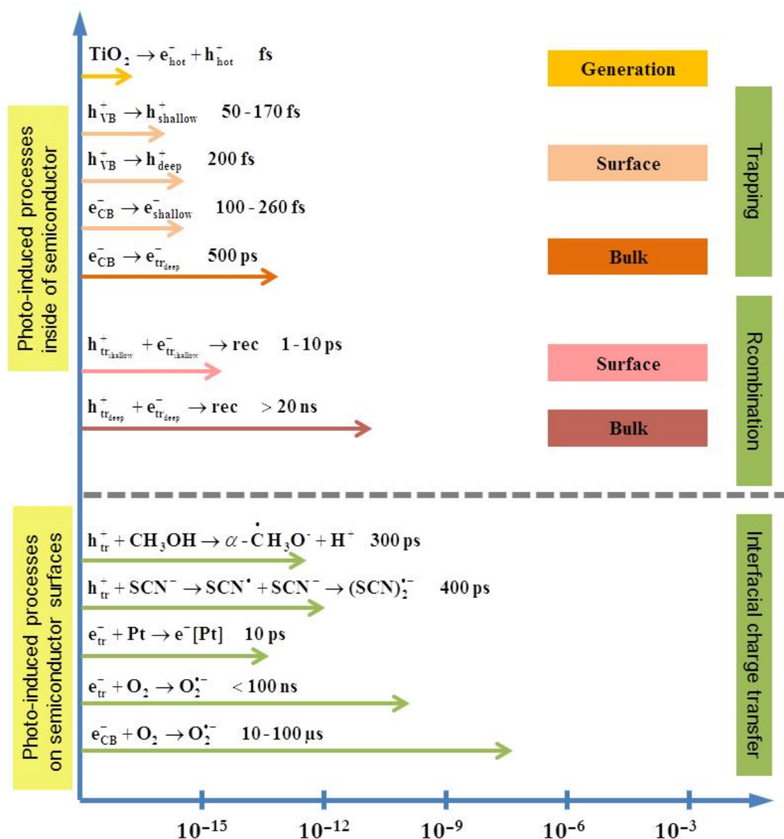
Scheme 1. Various steps involved in \text{TiO}_2 photocatalysis. Reproduced with permission from ref. [3] Copyright 2014 American Chemical Society
