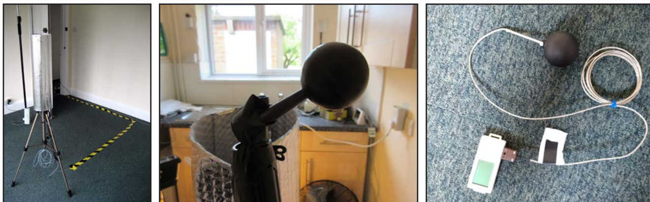
Figure 16. Left – shielded tripod covering wired U-type thermistor. Middle – 40 mm black globe on a U-type thermistor taped to a tripod. Right – battery powered T-type thermocouple.
