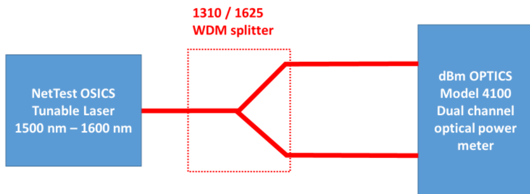
Figure 5-14 Block diagram of the experimental setup replicating the placement of a ratiometric power meter at the S s reference point (near the CWDM transmitter)
