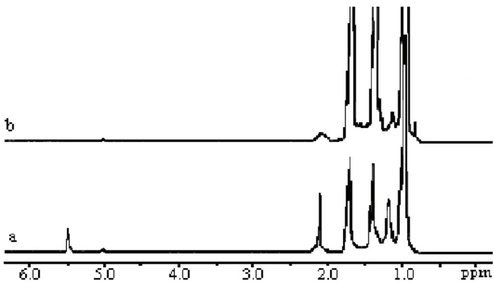
Figure 2 1 H-NMR spectra of PPB (a) and MPPB (b)
