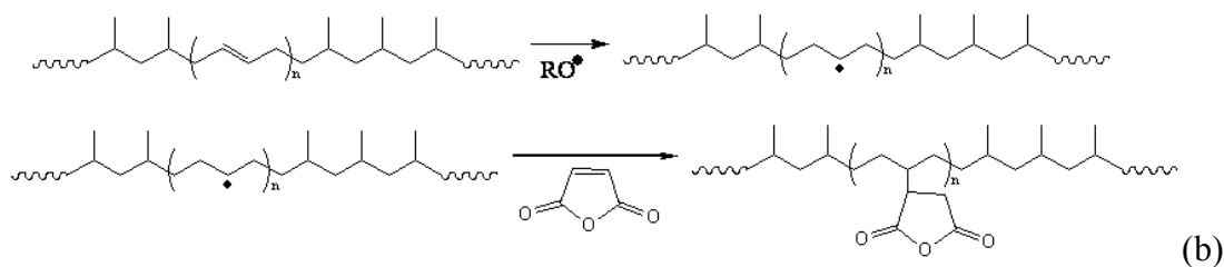
Scheme 1 Proposed reaction mechanisms for grafting maleic anhydride onto polypropylene (a) and polypropylene-butadiene copolymer (b)
