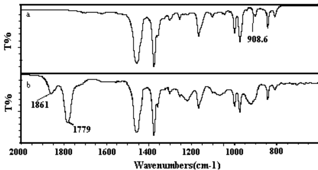
Figure 1 FT-IR spectra of PPB (a) and MPPB (b) from 2000 cm -1 to 600 cm -1 (MA = 14 wt%)
