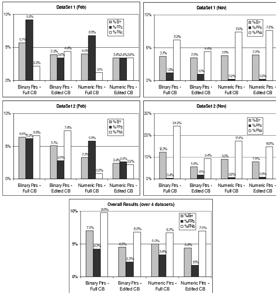
Figure 2. Results of evaluations for different feature representations
