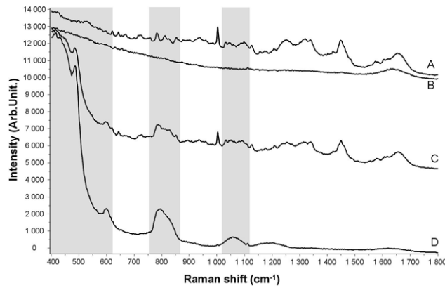
Fig. 1. Raman spectra recorded on different substrates. For each experiment an example of spectra recording from the cells is compared to the signal obtained from the corresponding substrate used (collagen gel or quartz). Spectra are offset for clarity. A: spectrum recorded from cells grown on collagen gel. B: background signal obtained from the Collagen gel. C: spectrum recorded from cells grown on quartz. D: background signal obtained from the quartz window.
