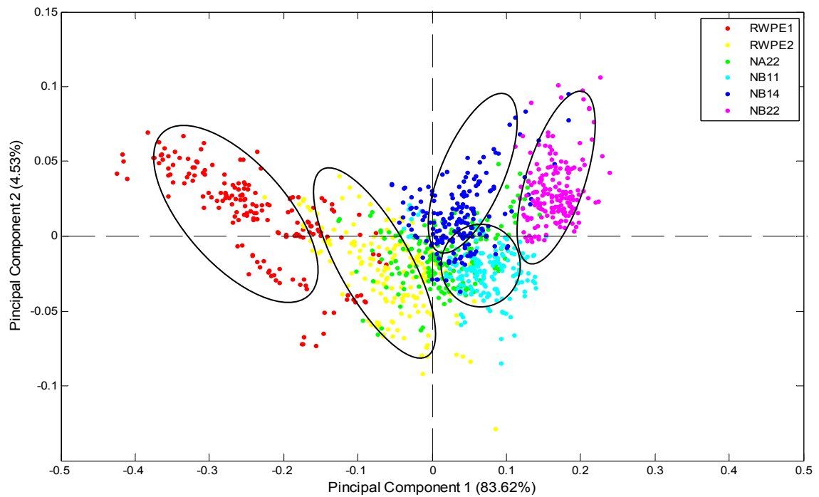
Figure 9. PCA score plot of the dataset processed using the optimum GA chosen pre-processing methods (PC1 vs. PC2). A different coloured circle as per the legend of the figure represents each spectrum of the cell lines (ellipses drawn as a guide to the eye).
