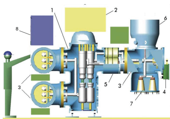
Fig. 1. Cross Section View of GIS
