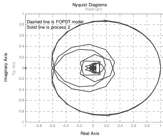
Figure 7: Nyquist plot for process (2), and FOPDT model of process (2).
