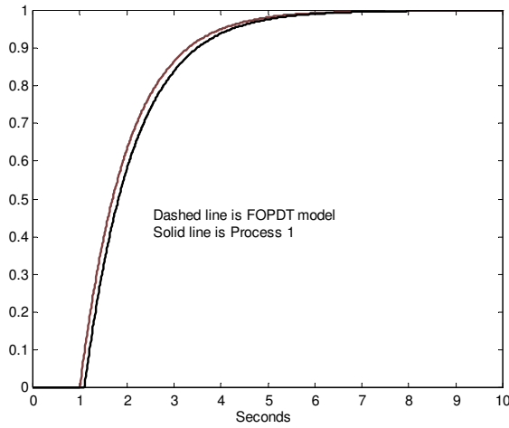
Figure 4: Open loop step response of process (1), and FOPDT model of process (1).
