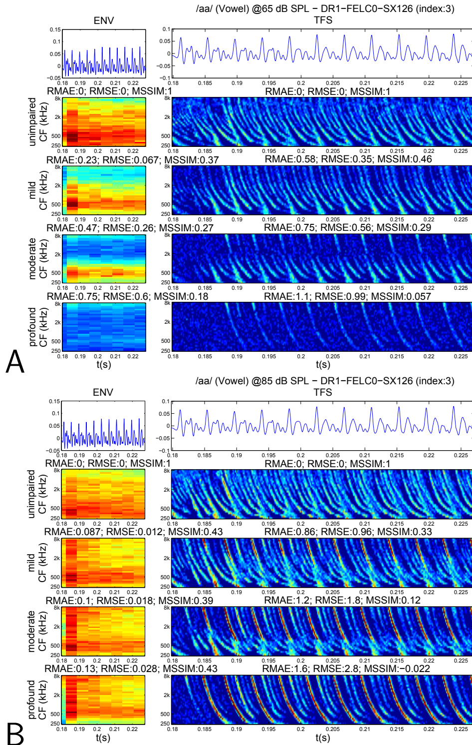
Figure 6: Corresponding samples to Fig. (5) ENV and TFS neurograms for a vowel (/aa/) with progressively degrading hearing loss. The TFS neurograms in (A) show that at lower presentation levels the vowel degrades with progressive hearing loss of fine timing information. In (B), it can be seen that at 85 dB SPL not only is information being lost, phase locking and a spread of synchrony across CF bands is causing the addition of erroneous information with progressive hearing loss.
