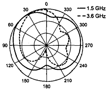
Figure 6. E-plane pattern for the simple HILA
