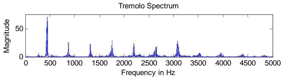
Figure 4.26: Spectrum of a tremolo sample.
