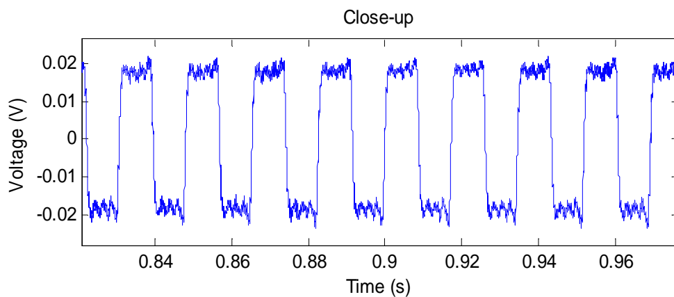
Figure 2.5: Helmholtz motion legato bow stroke.
