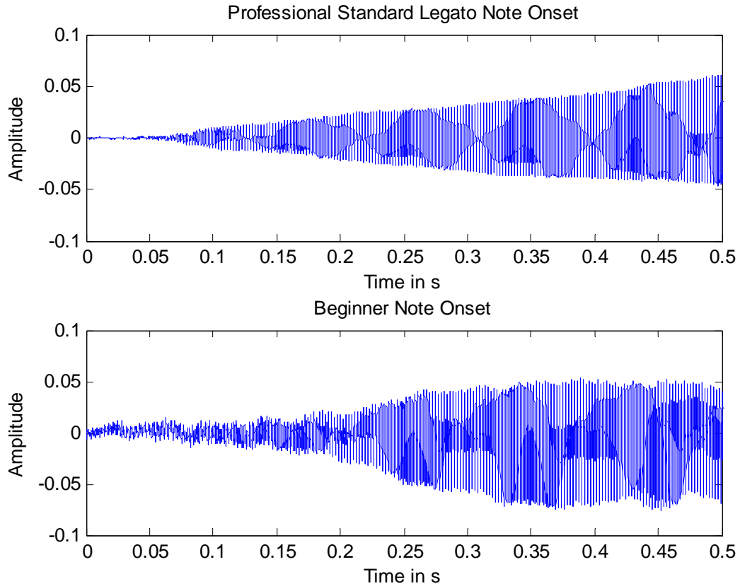
Figure 4.3: Professional standard legato (top) and beginner (bottom) note onsets.
