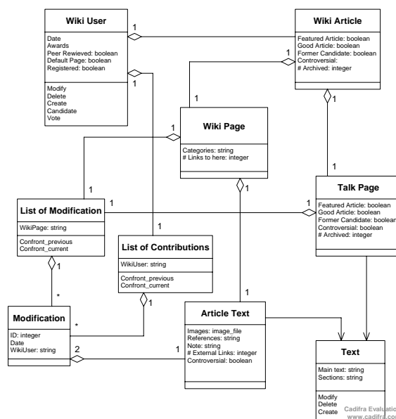
Figure 1 The Wikipedia UML model
