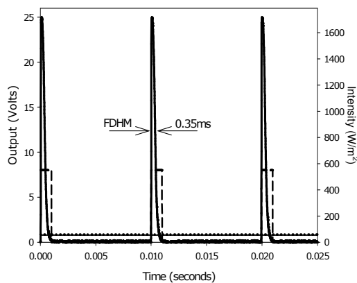
Figure 5 The pulsed output delivery of the Q-sun (—), the FDHM continuous equivalent of the Q-sun (.....), the continuous output of the Oriol (——) and the ideal 100 Hz pulse with a 10 % duty cycle of 1 ms (- - - -).
