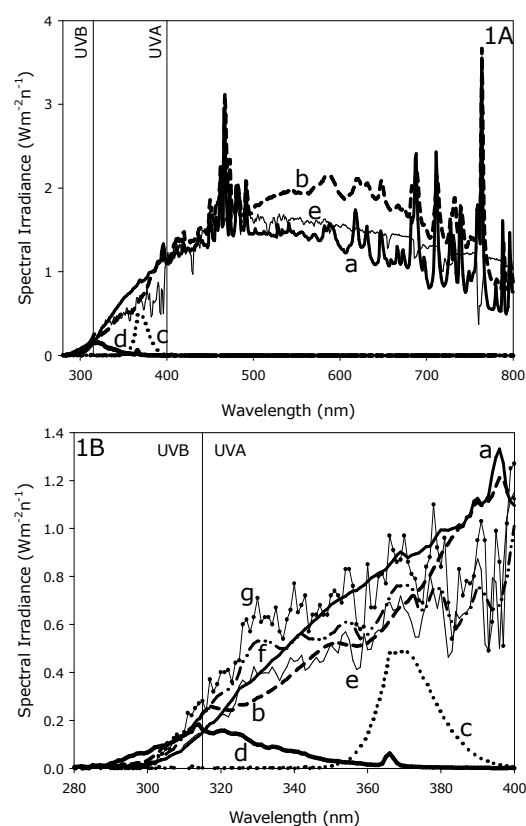
Figure 1 Spectral irradiance for the Q-sun solar simulator (a, \text{—} ), the Oriel solar simulator operating at 35 mA (b, \text{- - -} ), the UVA fluorescent lamp (c, \text{⋯⋯⋯} ), and the UVB fluorescent lamp (d, \text{—}\blacksquare\text{—} ) at their respective exposure levels shown alongside solar irradiance sampled midsummer in Naples Italy 40° N (e, \text{—} ) from 280 nm to 800 nm in (1A) and 280 nm to 400 nm in (1B). Also shown in (1B) are the irradiance spectra for solar radiation sampled midsummer in Albuquerque 38°N (f, \text{- - -}\blacksquare\text{- - -} ) and Melbourne 38°S (g, \text{—}\bullet\text{—} ) (30) .
