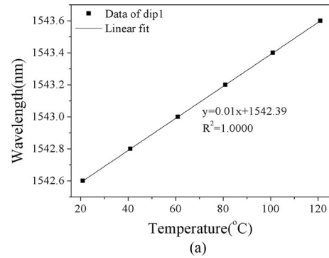
Fig. 12. Transmission spectrum response shift for different temperature.
