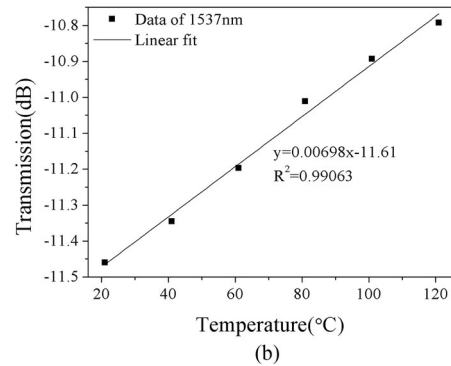
Fig. 13. (a) Dip wavelength shifts as a function of temperature; (b) Transmission as a function of temperature (at 1537 nm).
