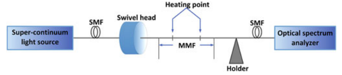
Fig. 5. Experimental setup for twist SMS fibre.
