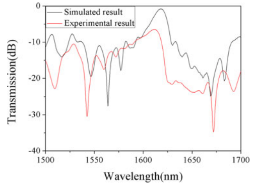
Fig. 6. Simulated data and experimental results of STMS fibre.
