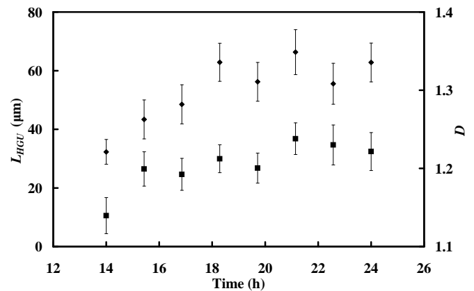
Fig. 3. Temporal variation in mean hyphal growth unit ( L_{HGU} ; ◆) and the mean fractal dimension ( D ; ■) of populations of A. oryzae cultivated on malt agar. Error bars represent 95% confidence intervals.
