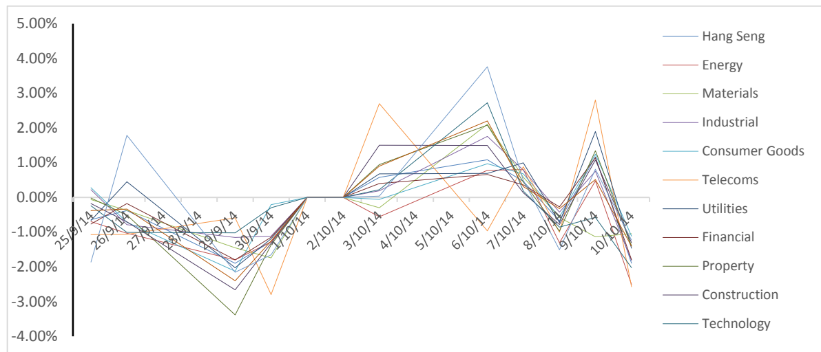
Figure 2: Hang Seng Index and Sectoral Changes
