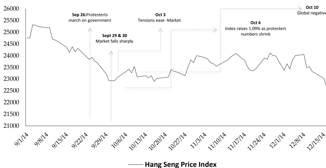
Figure 1: Hang Seng Index Performance during the Umbrella Protests
