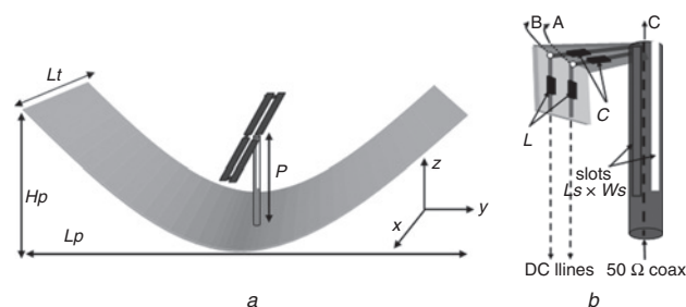
Fig. 2 Solar folded dipole antenna with parabolic reflector a Perspective view of proposed antenna with dimensions L_t = 205 mm, H_p = 75 mm, L_p = 245 mm for parabolic reflector with focal line at P = 55 mm b RF-DC decoupling network with dimensions L_s = 45 mm, W_s = 1.9 mm for slot illustrating balun on 50 \Omega line
