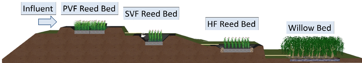
Fig 2 Longitudinal section through site at Lynch Lane
