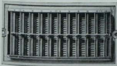
Multi-Shutter Damper—Type HC (Single Link)
